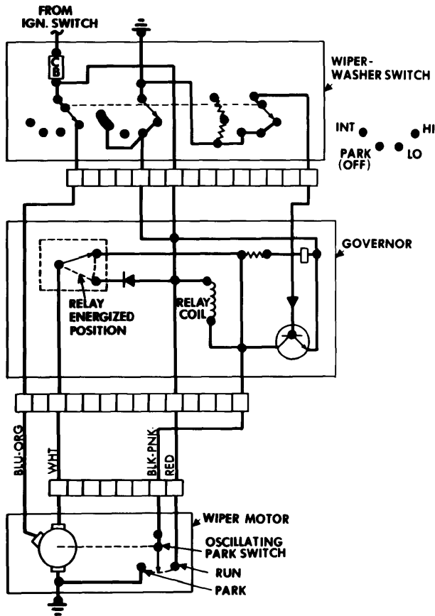
Ford Motor Co. Two-Speed Non-Depressed Intermittent Wiper System Wiring Diagram - Pinto, Bobcat, Maverick and Comet
