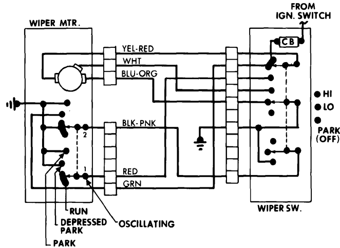
Ford Motor Co. Depressed Park Wiper System wiring Diagram (Exc. Intermittent Wipers) - LTD II, Cougar, Thunderbird, Ford, Mercury, Lincoln and Mark V
