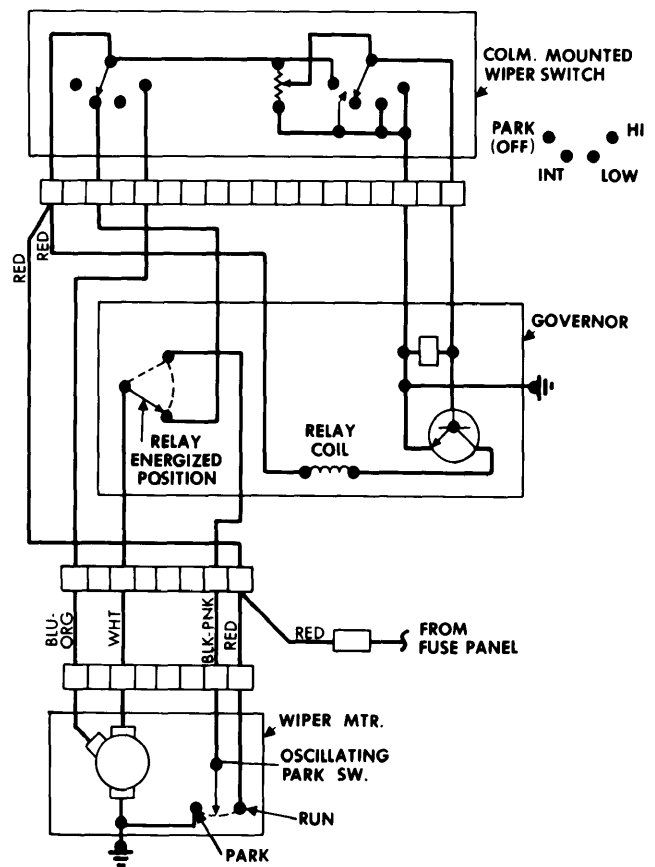
Ford Motor Co. Two-Speed Non-Depressed Intermittent Wiper System Wiring Diagram - Mustang, Granada and Monarch
